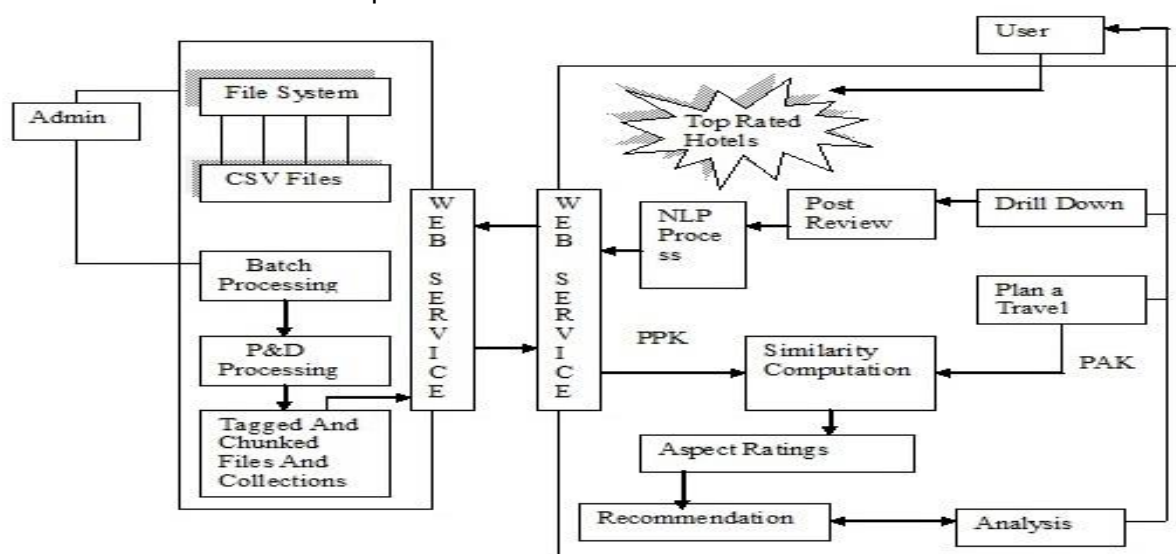
Fig. 1. Architecture Diagram: shows the architecture diagram.
